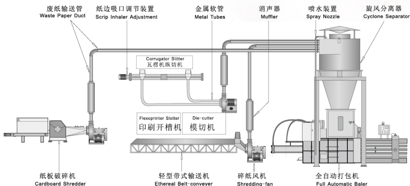
瓦楞纸箱行业整厂废纸处理系统示意图 The Diagram of Packaging Waste Management Systems
